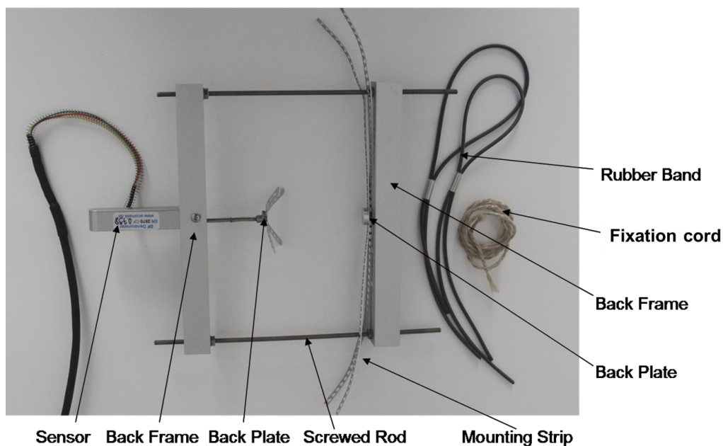
DF3 Fruit Dendrometer
