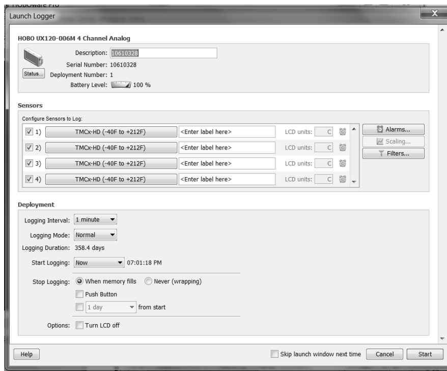
Fig. 5 Launch window
